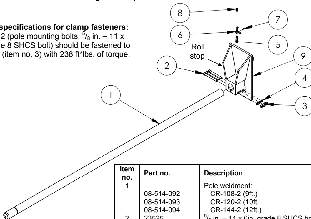
FIG. 1: Exploded parts diagram for Class 2 carriage CR-series carpet poles with welded lower carriage clamp
