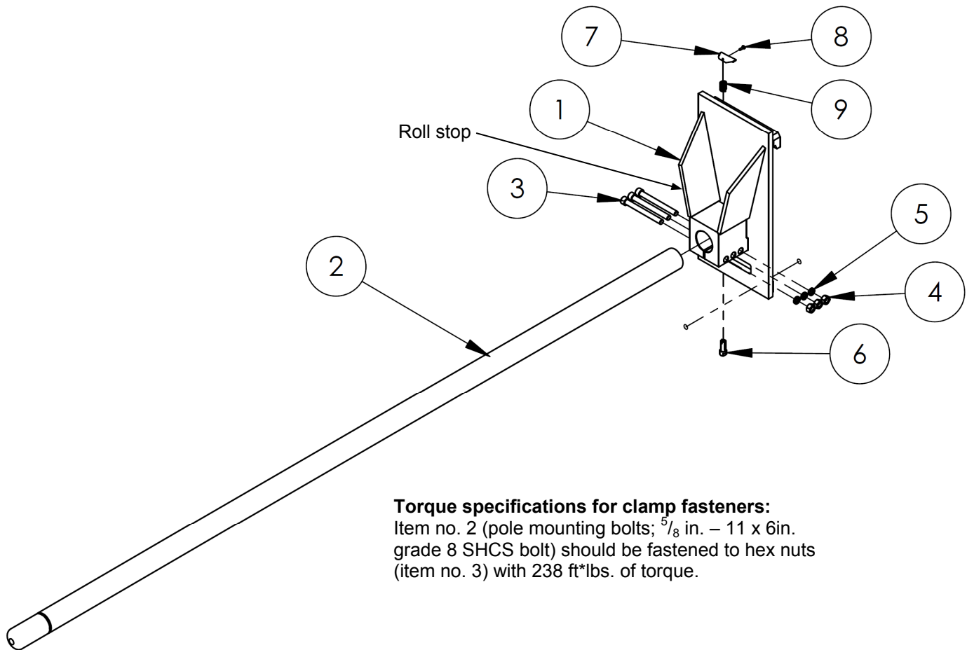
FIG. 2: Exploded parts diagram for Class 3 carriage CR-series carpet poles with welded carriage clamp
